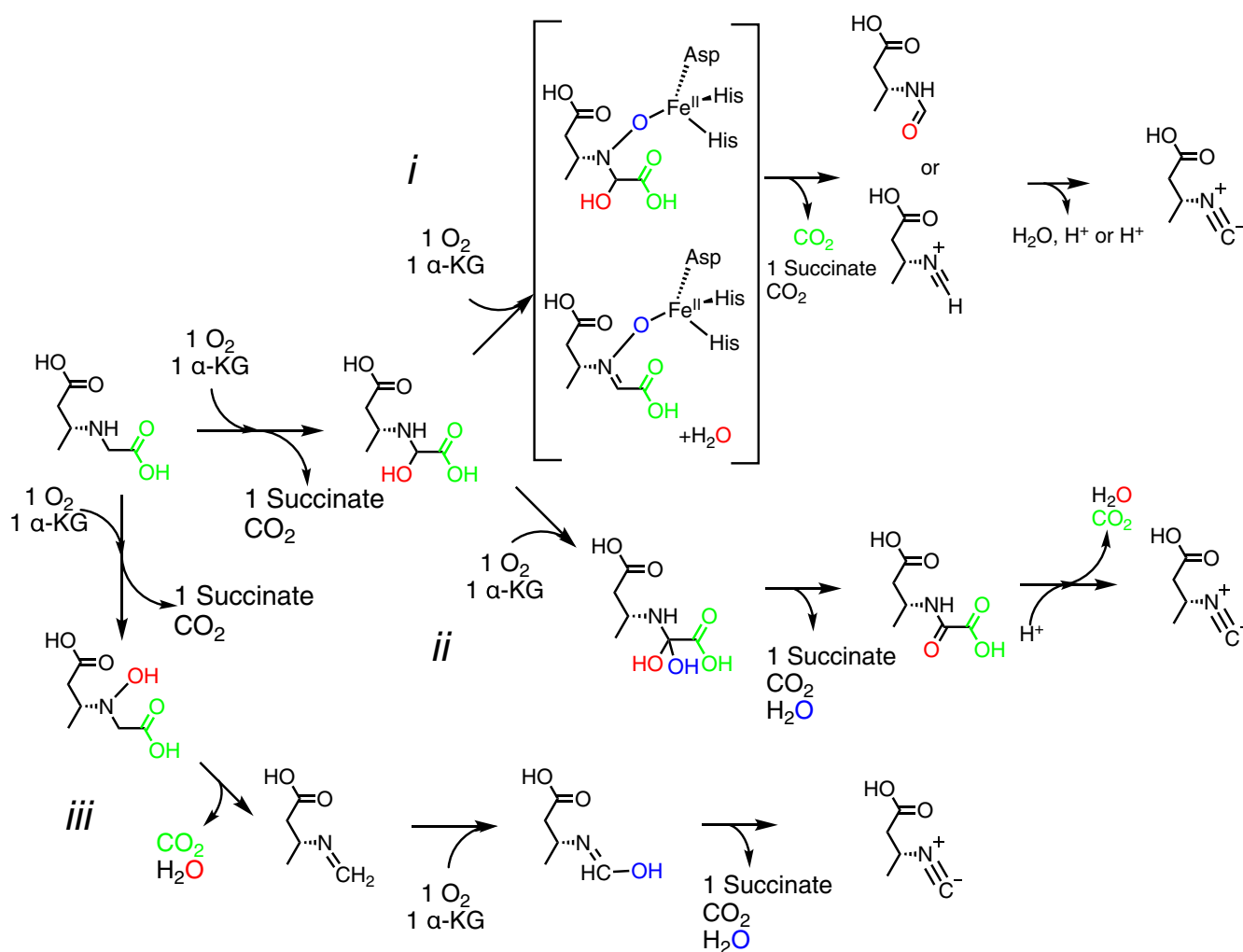
Figure 2. Possible mechanisms of isonitrile formation by ScoE. Top schemes ( i and ii ) show αKG-dependent hydroxylation at C5 of CABA occurring first. Schemes i and ii differ in the second half-reaction with αKG. These schemes are based on reaction mechanisms proposed by Chang and coworkers (13). In scheme iii , αKG-dependent hydroxylation of N occurs before αKG-dependent hydroxylation of C5 of CABA.
