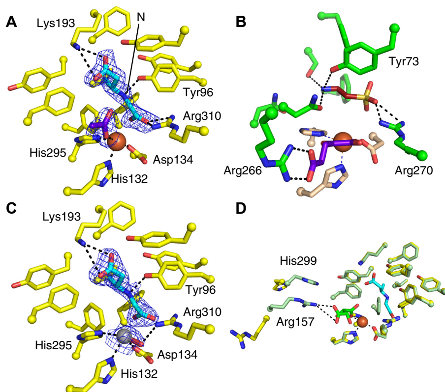
Figure 3. Active site comparisons. A, ScoE with CABA (cyan), Fe(II) (orange sphere), and acetate (purple). For clarity, the nitrogen atom of CABA is labeled. B, TauD (1O57) with taurine (red), \alpha -KG (purple), Fe(II) (orange sphere), and facial triad (wheat). C, ScoE with CABA (cyan) and oxovanadium (gray with oxygen atom in red). D, superposition of ScoE structures shows two positions of Arg157 and His299. The structures solved in this work are shown in yellow, the previously determined structure (with tartrate bound, PDB: 6L6X) is shown in green. CABA is shown in cyan, tartrate in purple, and Fe(II) as an orange sphere. Maps shown in blue mesh above are 2F_o - F_c composite omit maps contoured at 1\sigma . Dashed lines indicate close interactions (less than 4.0\text{ \AA} ).
