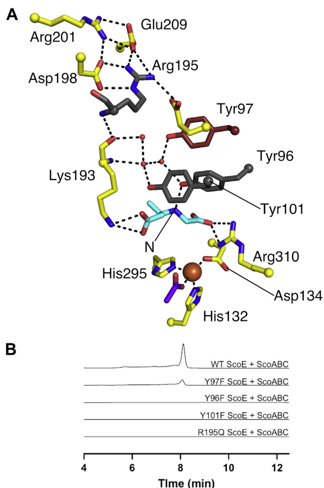
Figure 5. Hydrogen bonding network in ScoE extends from CABA to the protein surface. A, CABA is shown in cyan, acetate is shown in purple, and Fe(II) is shown as an orange sphere. Tyr96, Tyr101, and Arg195 are shown in gray, indicating that product is not detected when these residues are substituted. Tyr97 is shown in red to indicate that substitution of this residue results in reduced product formation. Dashed lines indicate close interactions (less than 4.0 Å). For clarity, the nitrogen atom of CABA is labeled. B, extracted ion chromatograms corresponding to the production of the INLP (calculated: [M + H]^+ = 323.2078 , observed: [M + H]^+ = 323.2093 , 4.6 ppm error) from coupled ScoABCE assays using wild-type ScoE and four single amino acid variants. In all cases, the calculated masses with a 10-ppm error tolerance were used. A reaction mixture comprised of 50 mM HEPES, pH 8, 500 \mu M \alpha -KG, 2 mM CABA, 100 \mu M Apo-ScoE, and 90 \mu M (\text{NH}_4)_2\text{Fe}(\text{SO}_4)_2 was gently mixed and incubated for 10 min at room temperature. After incubation, the reaction was mixed with 25 \mu l of 2 mM \text{MgCl}_2 , 5 mM ATP, 500 \mu M lysine, 4 mM NADPH, 50 \mu M ScoA, 50 \mu M ScoB, and 20 \mu M ScoC.
